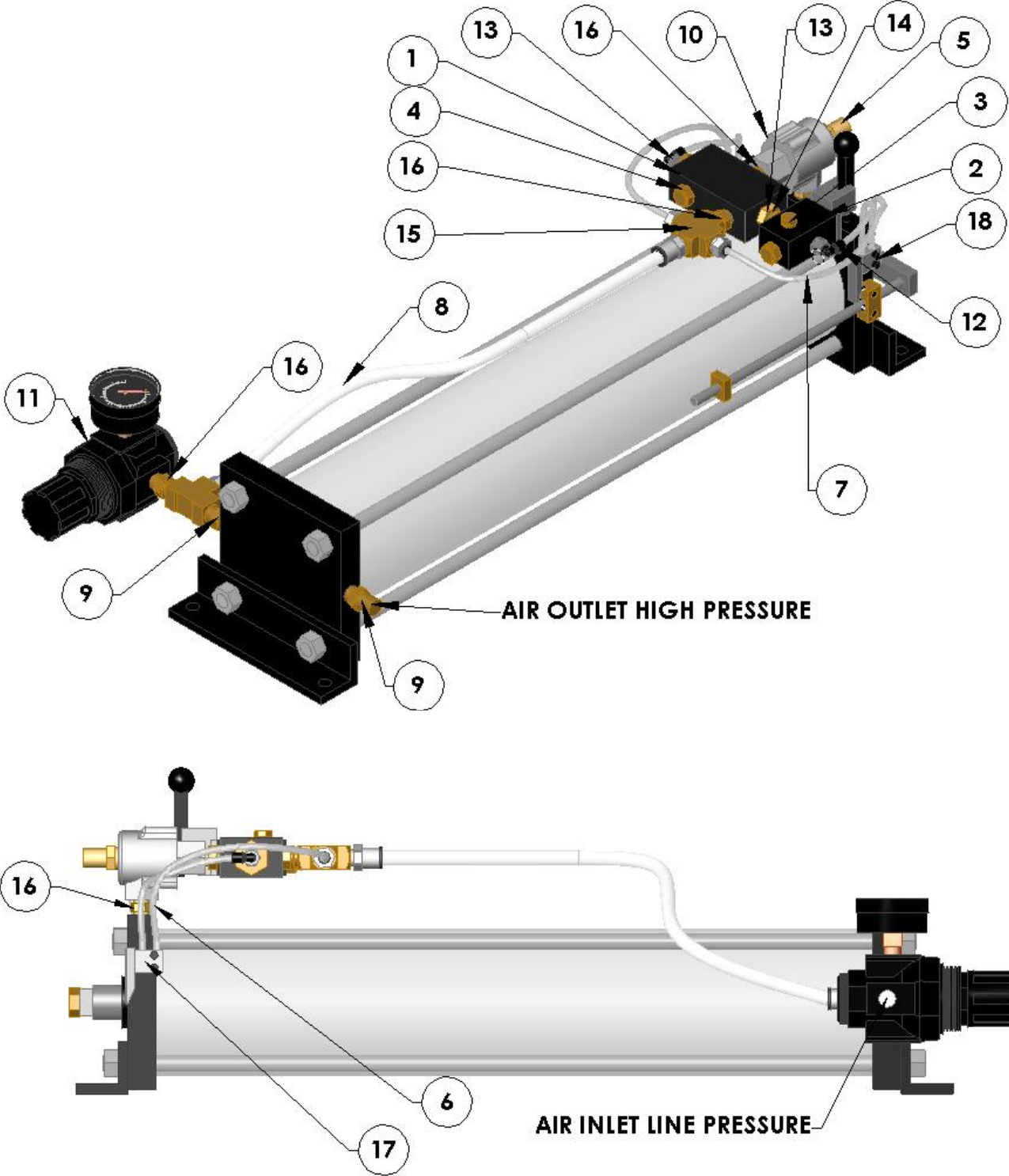
Fig. 19 Booster Pump (14799) part list
