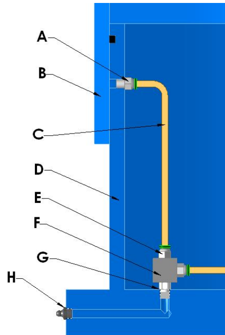
Fig. 11 Model HC Lubrication
