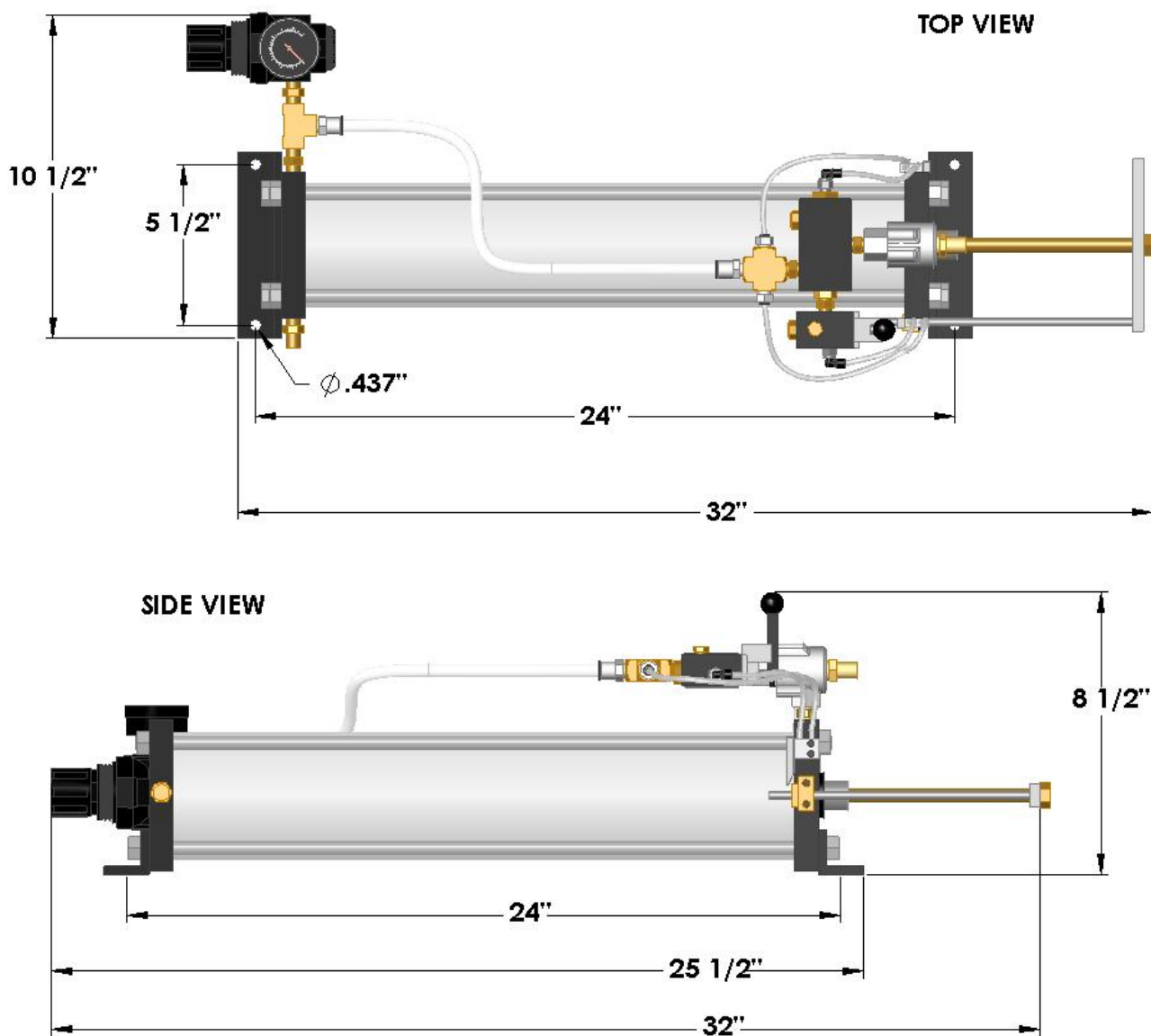
Fig. 18 Booster pump dimensions
