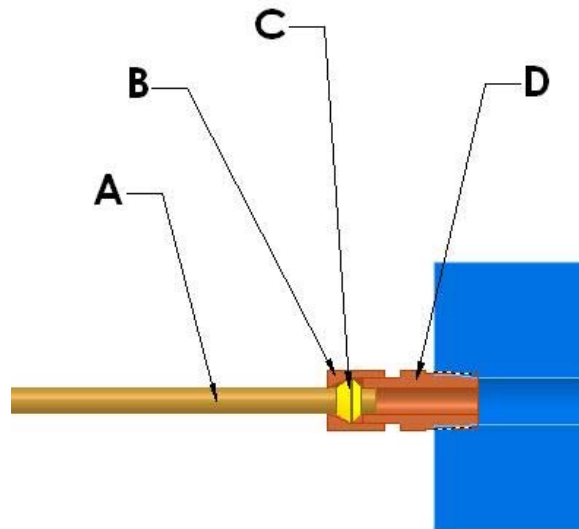
Fig. 14 Centralized lubrication fittings on the high pressure die cushion.
