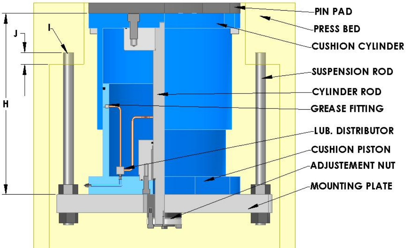
Fig. 6 Press bed mounted cushion. Dimensions A and B to be specified by the customer.
