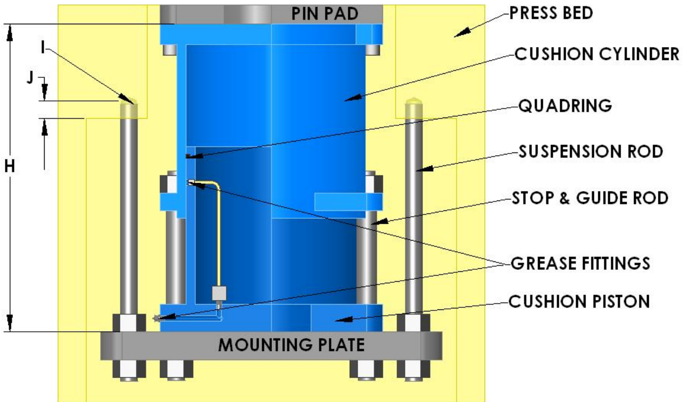
Fig. 6 Model HC Die Cushion – cross section view
