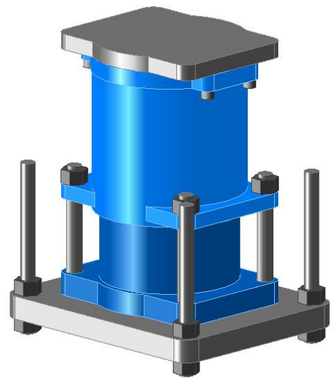
Fig. 5 Model HC Die Cushion 200 psi Max. Pressure
