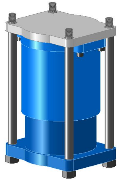
Fig. 3 Model HC Die Cushion 200 psi Max. Pressure
