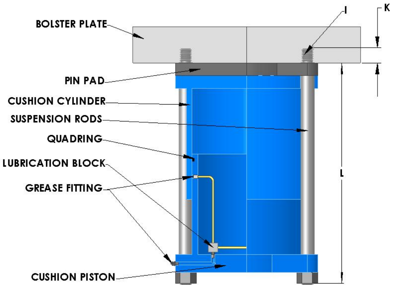
Fig. 4 Model HC Die Cushion – section and top view
