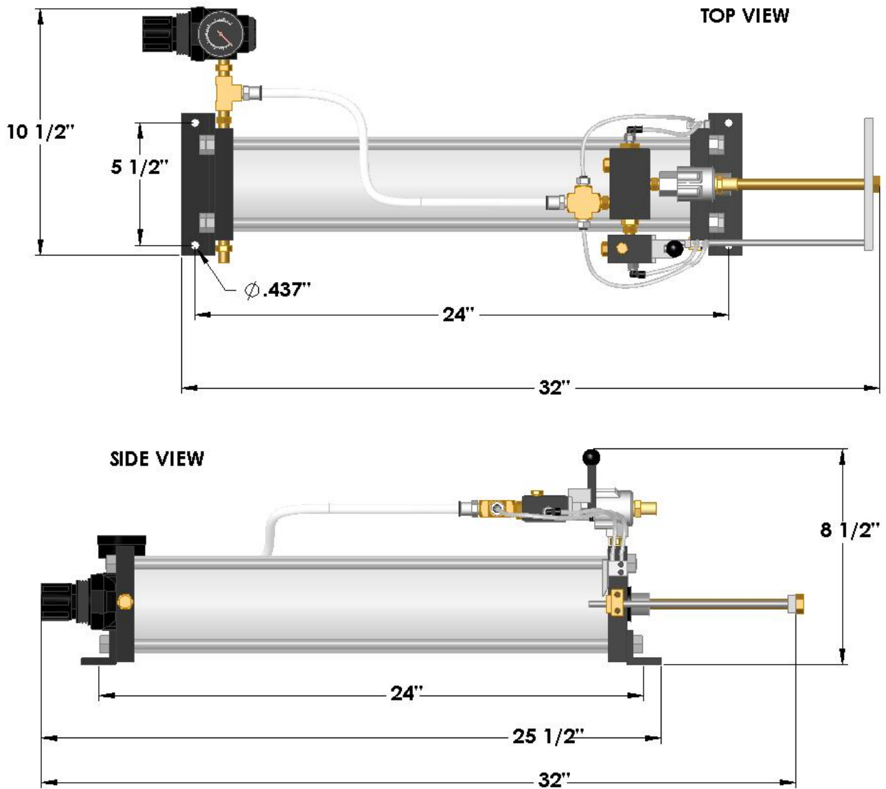
Fig. 18 Booster pump dimensions
