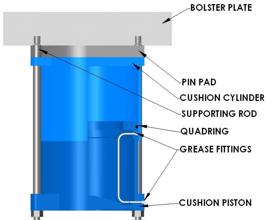
Fig. 1 Bolster Mounting
